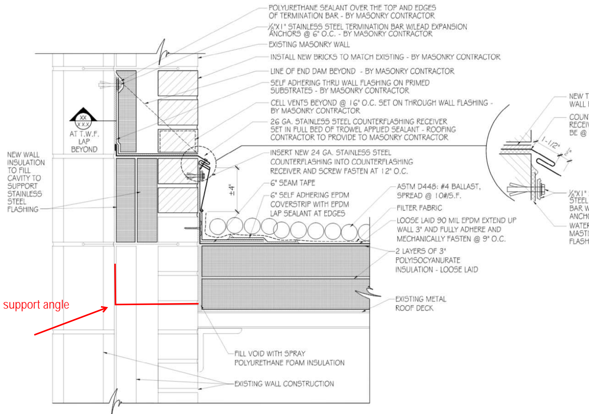
2 NEW THROUGH WALL FLASHING AND ROOF SYSTEM INSTALLATION DETAIL 3/8" = 1'-0"
